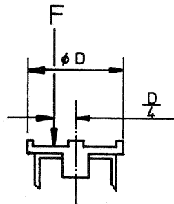
Figure B.3 - Load application for 2nd test
