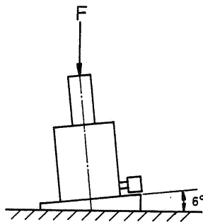
Figure B.2 - Stability Test
