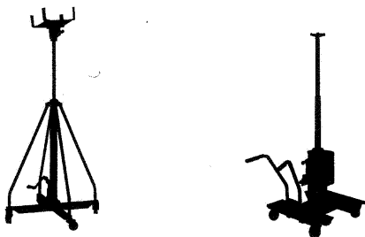
Figure 5 - Examples of hydraulic transmission jacks
