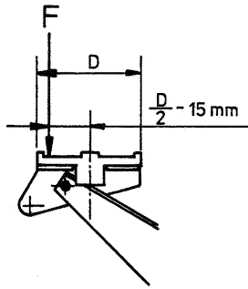
Figure B.7 - Load application for 5th test
