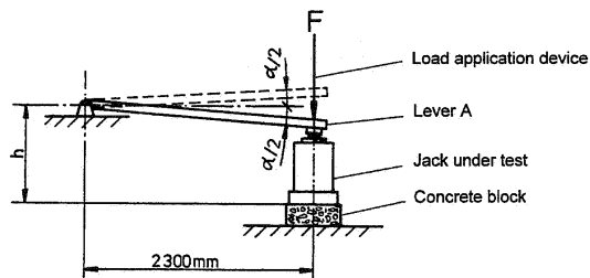
Figure B.1 - Test rig
