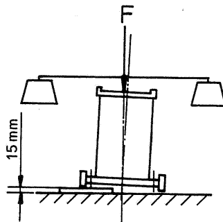
Figure B.6 - Load application for 4th test
