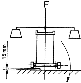
Figure B.5 - Load application for 3rd test
