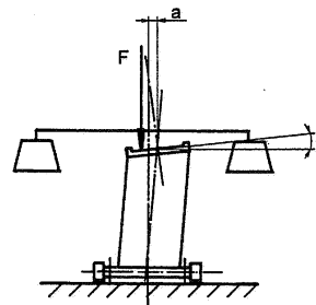
Figure B.4 - Load application for 2nd test
