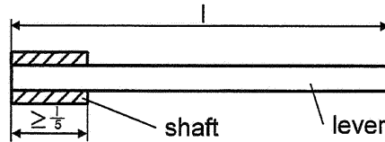
Figure 12 - Minimum length of lever in a shaft
