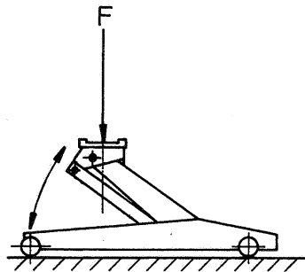
Figure B.9 - Load application for 6th test
